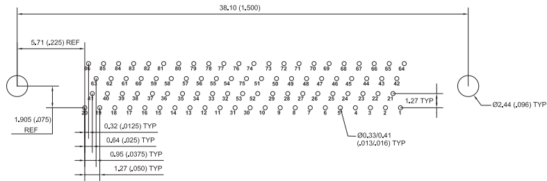
86 CONTACTS - VIEW B
