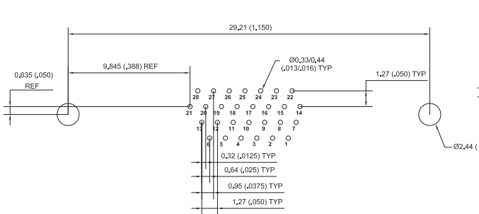
28 CONTACTS - VIEW B
