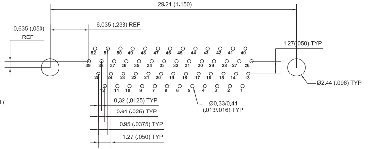
52 CONTACTS - VIEW B
