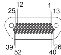
52 NANO WAYS IN A 15 WAY MICRO INSERT
