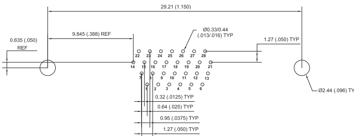
28 CONTACTS - VIEW B
