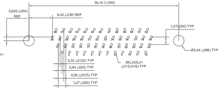
52 CONTACTS - VIEW B
