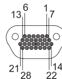
MATING FACE OF FEMALE CONNECTOR
