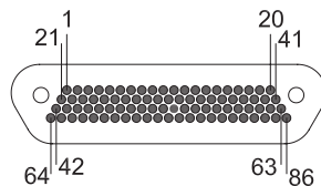
86 NANO WAYS IN A 25 WAY MICRO INSERT
