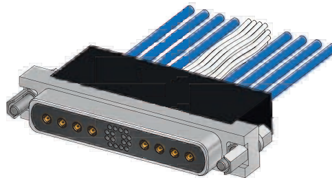
8 COAXIAL COMBO CONTACTS + 16 SIGNALS IN A 120 WAY MICRO-D CONNECTOR
