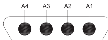
4 CONTACTS Ø3MM IN A 51 WAY MICRO-D SHELL
