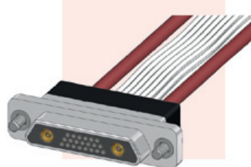
▲ COMBO 51 2 COAX S3 + 21SIGN MALE PIGTAIL
