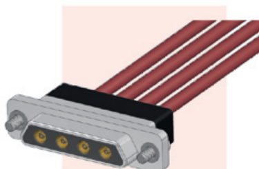
▲ COMBO51 4 COAX S3 MALE PIGTAIL
