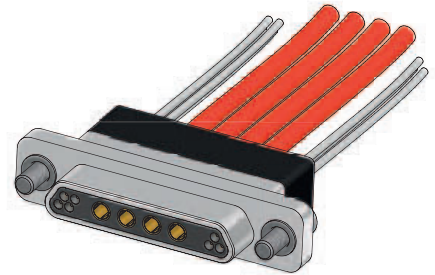
4 POWER COMBO CONTACTS + 7 SIGNALS
