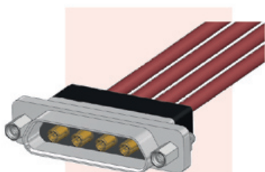
▲ COMBO 51 4 COAX S3 FEMALE PIGTAIL
