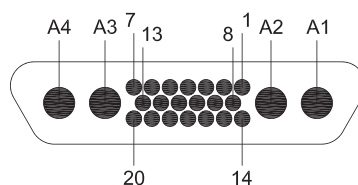
4 CONTACTS Ø2.2MM + 20 SIGNALS IN A 51 WAY MICRO-D SHELL
