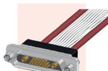
▲ COMBO 51 2 COAX S3 + 21 SIG FEMALE PIGTAIL
