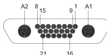
2 CONTACTS Ø3MM + 21 SIGNALS IN A 51 WAY MICRO-D SHELL
