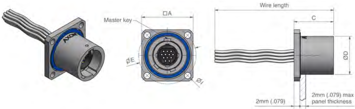
Rear mount square flange female MCABKxxx-00Sxxxxxx
