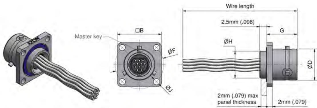
Front mount square flange female
