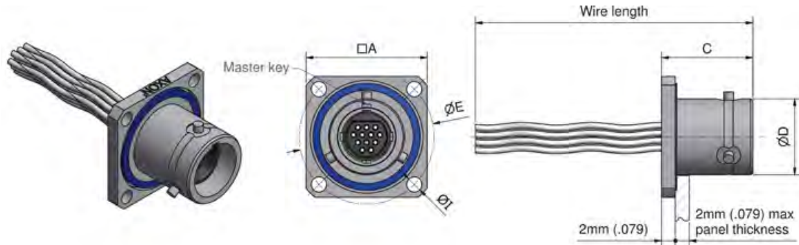
Rear mount square flange female
