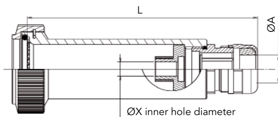
Backshell Type 3
