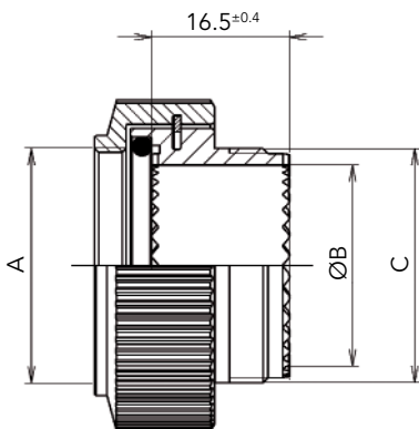
Backshell Type 1
