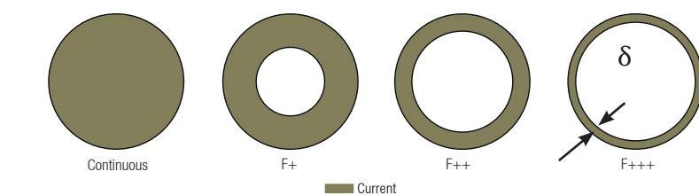
SKIN EFFECT
