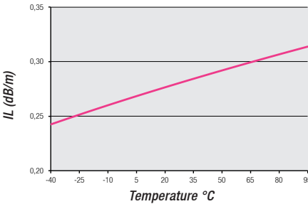
Insertion loss by temperature at 7 GHz
